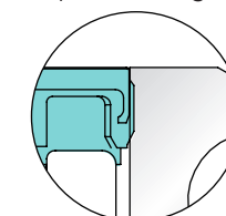
Bolt-Hole without Chamfer (optional: /TR)
