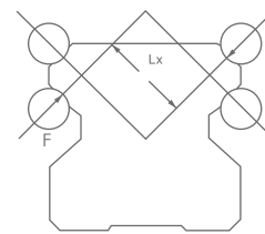
X-Type Arrangement
