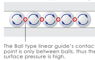
Traditional Ball type linear guide
