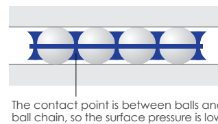
Low noise ball chain
