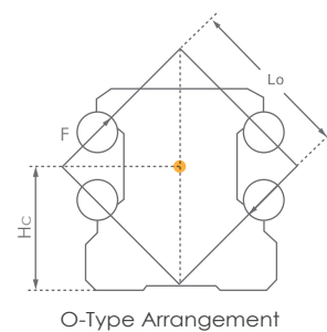
O-Type Arrangement
