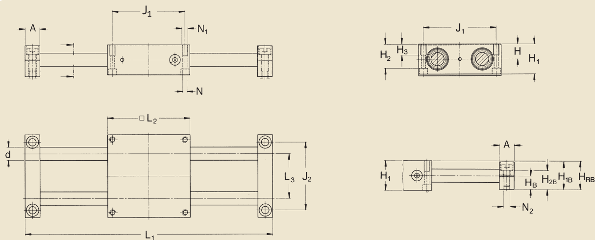
Design LZBU ... B with closed linear bearing unit
