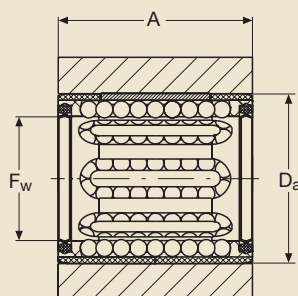
LTDR With double lip seals
