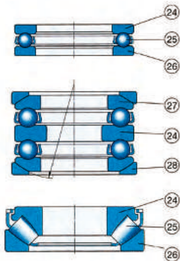
Thrust bearings (fig. 3)
