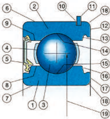
Radial bearings (figs. 1 and 2)
