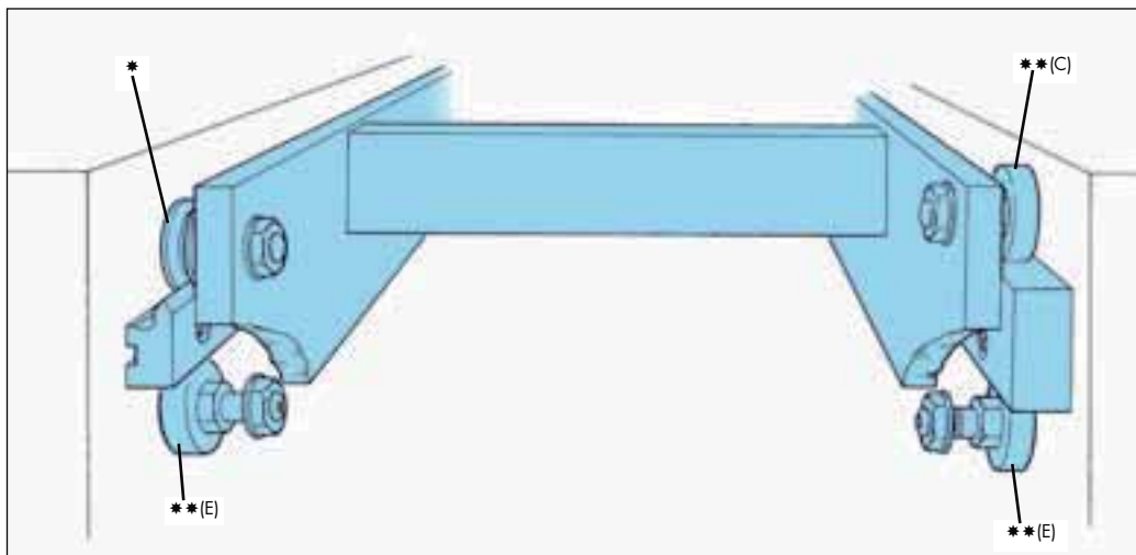
* Through Hole Fixing Slimline Bearing (Concentric) ** Narrow Track Roller (Concentric 'C' & Eccentric 'E')
