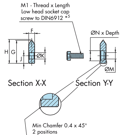
Slide with Standard Holes Slide with Counterbored Holes
