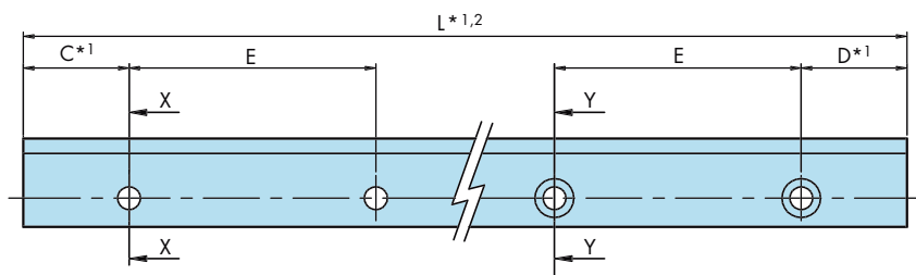
Slide with Standard Holes Slide with Counterbored Holes
