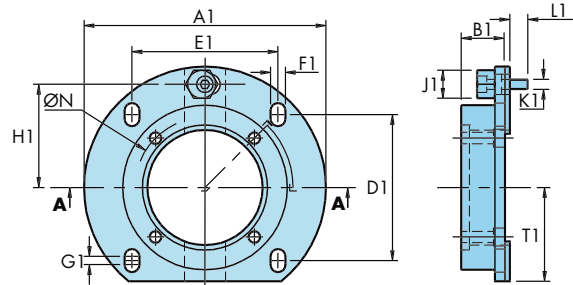
Drive Flange
