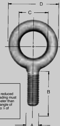
EYEBOLTS PLAIN PATTERN
